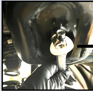
Installing the Finger Touch / EZ Drain Valve" with a 22mm wrench.
